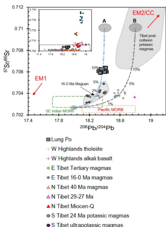
Figure 14. Plots of ^{87}\text{Sr}/^{86}\text{Sr} vs. ^{206}\text{Pb}/^{204}\text{Pb} isotopic mixing model for the Lung Po basalts. The (Pacific or Indian) MORB, for example, serves as a critical endmember. Mixtures of an (N) MORB with a series of sediments (e.g., Cousens et al., 1994) may explain most high-Pb isotope post-collision 42–24 Ma high-K magmas. However, mixing between a moderate-Pb isotope sediment (e.g., pelagic sediment in the SW sub-basin of EVS/SCS) with a low-Pb isotope Indian (I-) MORB) may explain the formation of the Lung Po and Maguan moderate-Pb and high-Sr isotope samples. Isotopic and elemental values of endmembers used in the mixing model are Pb (ppm), Sr (ppm), ^{206}\text{Pb}/^{204}\text{Pb} , and ^{87}\text{Sr}/^{86}\text{Sr} , respectively, for an I-MORB-like: 0.2, 25, 18.0, 0.70265; for a SW sub-basin of EVS/SCS: 20, 180, 18.4, and 0.710 (Line A), and a Pacific Ocean-like sediment: 17, 180, 18.8, and 0.710 (Line B). The inserted diagram illustrates the enrichment magnitude of North and South Tibet post-collision high-K magmas. See text for explanations
