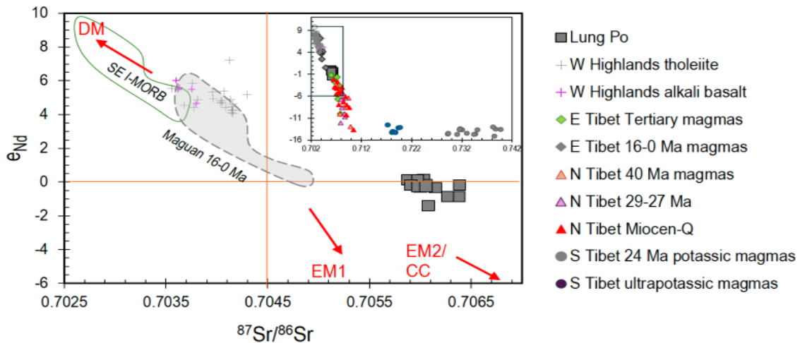
Figure 6. Plots of ^{87}\text{Sr}/^{86}\text{Sr} vs. \epsilon_{\text{Nd}} show the Lung Po Pleistocene basalts are much more EM2 enriched than Vietnam's contemporaneous Western Highlands and Maguan basalts; however, they all are much depleted than the Tibet 42–24 Ma high-K magmas (inserted diagram). The SE I-MORB data are from Mahoney et al. (2002). The other sources of data fields are as in Fig. 3. The mantle isotopic components (EM1: enriched mantle type 1, EM2: enriched mantle type 2; DM: depleted mantle) are after Zindler and Hart (1986)
