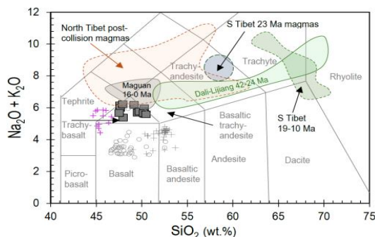
Figure 3. \text{Na}_2\text{O} + \text{K}_2\text{O} vs. \text{SiO}_2 (TAS) classification diagram for the Lung Po basalts (filled square) (e.g., Le Bas et al., 1986), plotted are Vietnam's Western Highlands Pleistocene tholeiite (gray cross) and alkaline basalt (pink cross; Hoang et al., 2019), and SE I-MORB (empty circle; Neal et al., 2002); also plotted for reference are data field of North Tibet 42–24 Ma high-K magmas (Guo et al., 2006), South Tibet 23 and 19–10 Ma magmas (Liu et al., 2014), and Dali-Lijiang 42–24 high-K magmas and Maguan 12–0 Ma basalts (after Wang et al., 2001)
