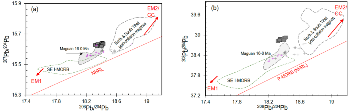
Figure 7. Plots of ^{206}\text{Pb}/^{204}\text{Pb} vs. ^{207}\text{Pb}/^{204}\text{Pb} (a) and ^{206}\text{Pb}/^{204}\text{Pb} vs. ^{208}\text{Pb}/^{204}\text{Pb} (b) show the Lung Po Pleistocene basalts are higher ^{207}\text{Pb}/^{204}\text{Pb} and ^{208}\text{Pb}/^{204}\text{Pb} at the same ^{206}\text{Pb}/^{204}\text{Pb} than other regional contemporaneous basalts. Sources for reference data fields are as in Fig. 2. NHRL (Northern Hemisphere Reference Line) is after Hart (1988) based on Pacific MORB (after White et al., 1987)
