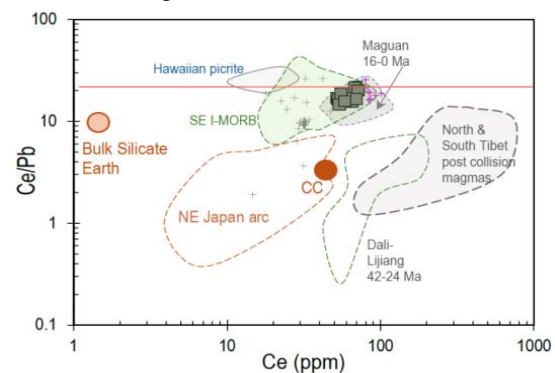
Figure 10. Plots of Ce/Pb vs. Ce for volcanic rocks from various tectonic settings showing Lung Po along with Maguan, Vietnam's Western Highlands, SE I-MORB and Hawaiian (after Norman and Garcia, 1999) magmas plot in the mantle-derived field separated from subduction-related (Kimura and Yoshida, 2006) and crustal related, e.g., Bulk Silicate Earth and Continental Crust (CC) (after Rudnick and Fountain, 1995; McLennan, 2001)
