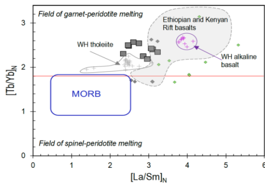
Figure 12. Plots of [La/Sm]_N vs. [Tb/Yb]_N for the Lung Po (filled square) and Maguan 16–0 Ma basalts (gray filled diamond), and 42–24 Ma high-K magmas (green filled diamond) (after Wang et al., 2001). Mantle plume-derived Ethiopian and Kenyan fields are from Furman et al. (2004), Vietnam's Western Highlands (WH) tholeiitic and alkaline basalts are from Hoang et al. (2019). Data for SE Indian MORB are from Neal et al., 2002. In theory, except for the MORB, all the plotted basalts were derived from the field of garnet peridotite melting. Chondrite normalizing data are from Sun and McDonough (1989)
