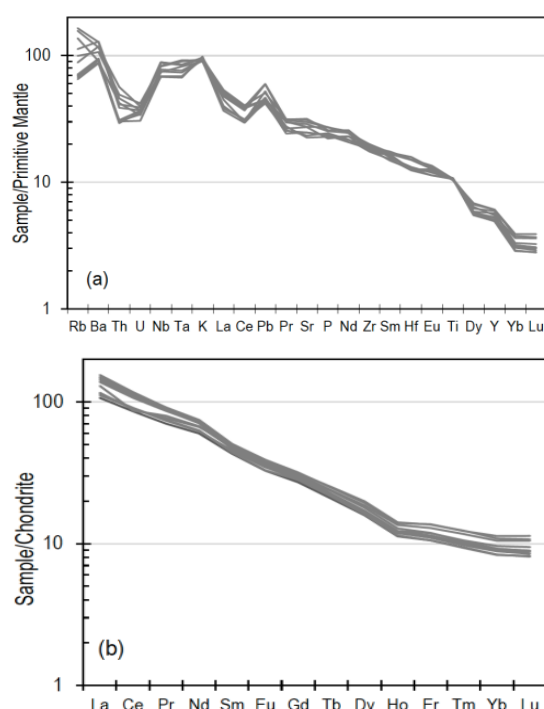
Figure 5. (a) The primitive mantle trace element normalization patterns for the Lung Po basalts, except for the Th and U troughs, are essentially oceanic island basalt-type (normalizing data are from Sun and McDonough, 1989); (b) The chondrite rare earth element (REE) normalization configuration of the Lung Po basalts shows a sharp decrease from the light (L)-REE to middle (M-) and heavy (H-) REE, reflecting a significant depletion of HREE relative to LREE (after Sun and McDonough, 1989)
