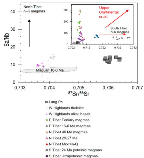
Figure 9. Correlation between ^{87}\text{Sr}/^{86}\text{Sr} and Ba/Nb shows Lung Po and Maguan basalts do not correlate positively with Ba/Nb, suggesting no apparent crustal contamination. In contrast, North Tibet high-K magmas display high Ba/Nb, reflecting the influence of hydrous fluids, while South Tibet magmas with very high ^{87}\text{Sr}/^{86}\text{Sr} , suggesting crustal melt influence (inserted diagram). Sources of data fields are as in Fig. 2. See text for explanation
