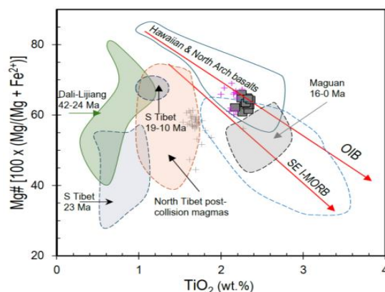
Figure 11. Plots of \text{Mg\#} [=100 \times (\text{Mg}/(\text{Mg} + \text{Fe}^{2+}))] vs. \text{TiO}_2 shown are fields of crustally influenced North and South Tibet post-collision 42–24 Ma high-K magmas (after Wang et al., 2001; Guo et al., 2006; Liu et al., 2014). Mantle-derived references include SE I-MORB, Hawaiian, and North Arch magmas (Norman and Garcia, 1999; Frey et al., 2000), Lung Po, Maguan, and Vietnam's Western Highlands basalt. See text for explanations
