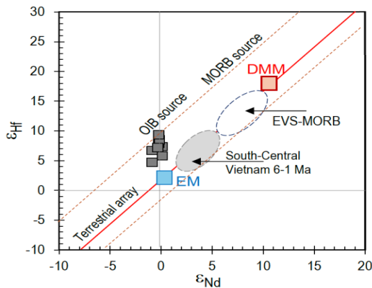
Figure 8. Plots of \epsilon_{\text{Hf}} vs. \epsilon_{\text{Nd}} show the Lung Po basalts are more enriched in ^{143}\text{Nd}/^{144}\text{Nd} (expressed by \epsilon_{\text{Nd}} ) relative to ^{176}\text{Hf}/^{177}\text{Hf}
