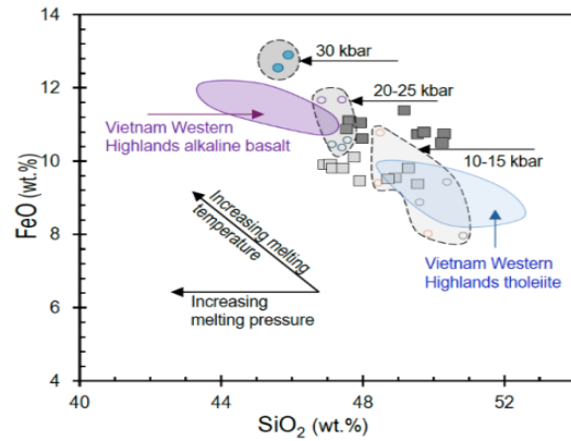
Figure 13. Plots of (wt.%) SiO 2 vs. FeO of the Lung Po basalts (black square) and their primitive melts' chemical compositions (gray square) calculated after Putirka (2008). The experimental peridotite melting pressures of fertile peridotite HK-66 and refractory KBL-1 are after Hirose and Kushiro (1993). Arrows indicate progressive partial melting from low- to high temperature and pressure. Except for a few samples in upper corner of 10–15 kilobars (kb) field, most 'primitive' Lung Po basalts plot in the 20–25 kb field
