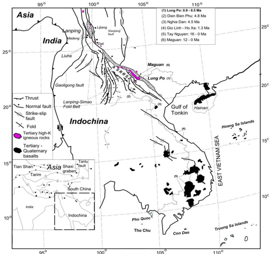
Figure 1. The scheme of India-Eurasian collision and distribution scheme of post-collision volcanism and regional faults in China and Vietnam are simplified after Wang et al. (2001) and Hoang and Flower (1998). The ages of Maguan basalts are from Wang et al. (2001) and Xie et al. (2021); the Lung Po basalts' ages are from this study; other Vietnamese basalts are from Hoang and Flower (1998). ASRRSZ: Ailao Shan Red River Shear Zone
